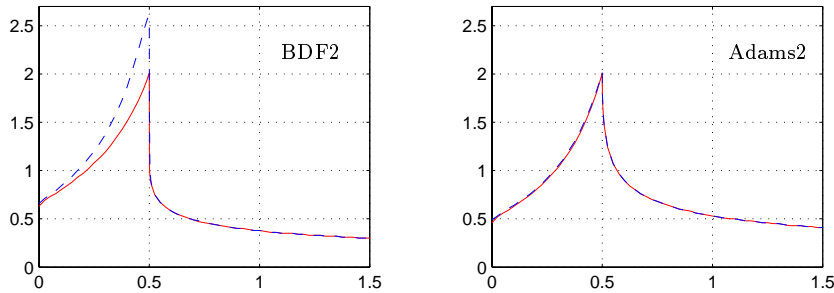
FIG. 5.2. Positivity test for the implicit two-step methods (3.17) with \xi = \frac{2}{3} [left] and \xi = 1 [right]. Courant numbers versus \eta \in [0, \frac{3}{2}] , starting with backward Euler [dashed lines] and method (3.19) [solid lines].
