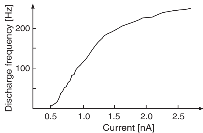
B. Gain function of hippocampal pyramidal neuron
