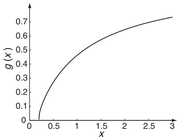
A. Gain function for population average in adiabatic limit
