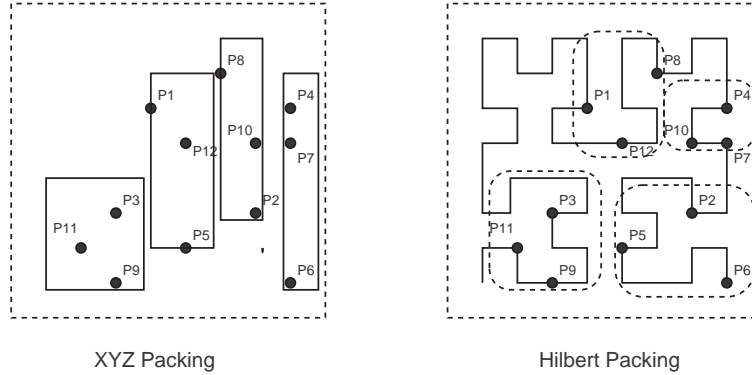
Figure 2. Hilbert curve packing versus XYZ.
