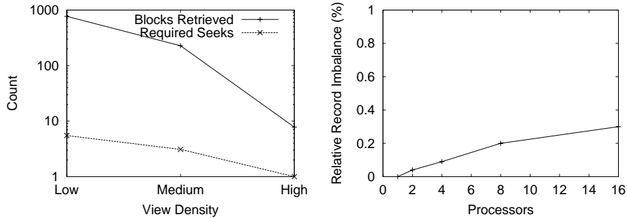
Figure 6. (a) Disk blocks received vs. number of disk seeks required on 16 processors, and (b) Relative record imbalance percentage.
